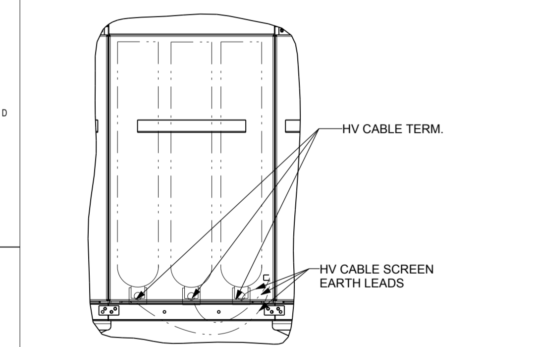
DETAIL B SCALE 0.100 Q FUNCTION TX-HV CABLE SCREEN EARTHING ARRANGEMENT INSIDE CABLE BOX
