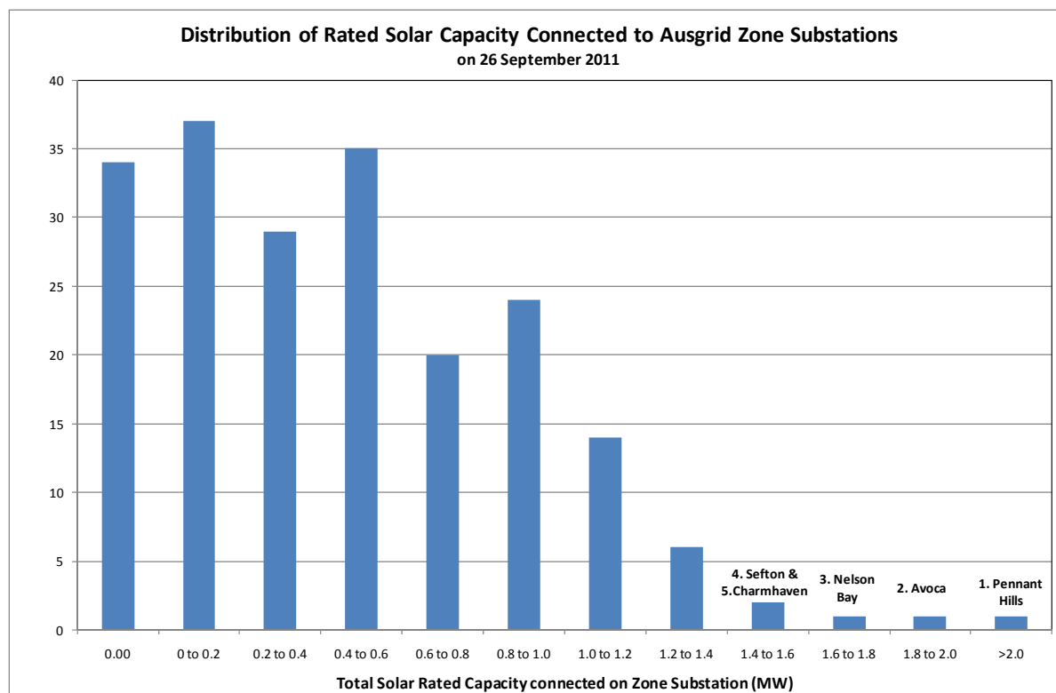
Figure 4: Rated solar capacity connected by Zone Substation
