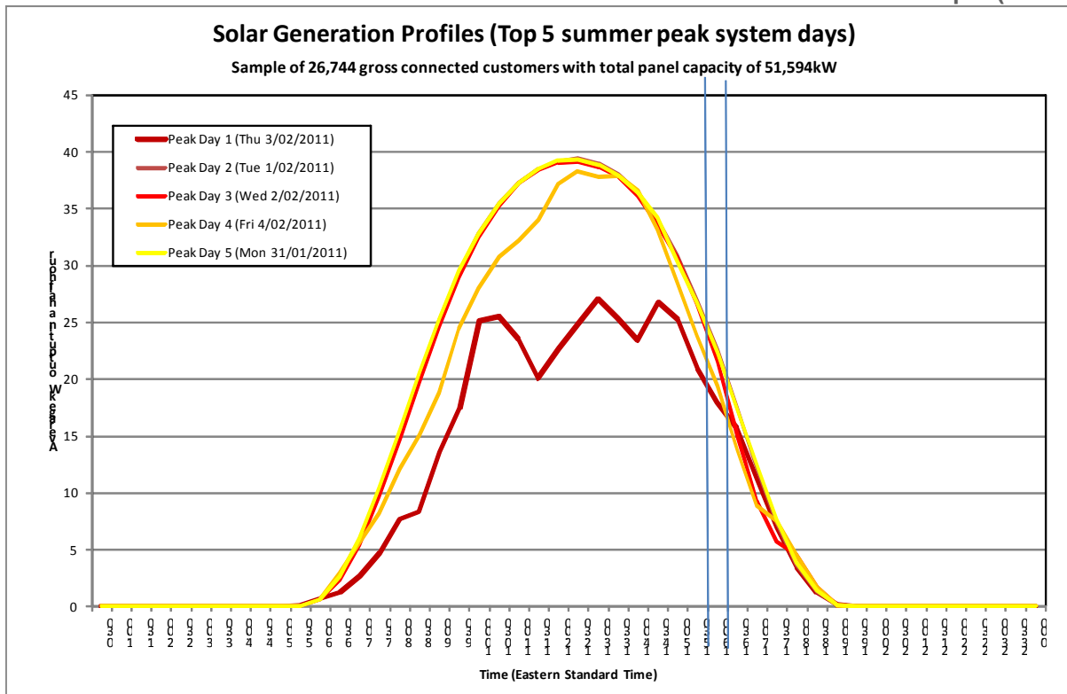
Figure 3: Ausgrid network total solar gross generation – top five summer days in 2011
